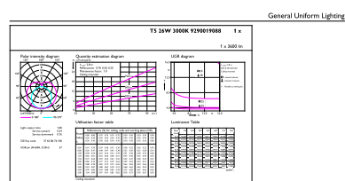
CalcuLux Photoemetrics 4.5 Philips Lighting B.V. Page: 1/1
