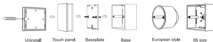
Installation diagram:
