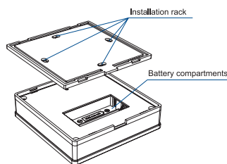
Installation diagram:
