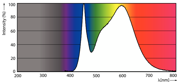
Spectral Power Distribution Colour - LEDbulb ND 10-75W A60 E27 840 1CT
