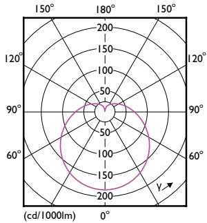
Light Distribution Diagram - LEDbulb ND 8-60W A60 E27 827 1CT
