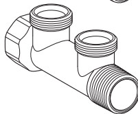
602.422.00.1, Rg, R 3/4" / Rp 3/4" 612.422.00.1, Ms, R 3/4" / Rp 3/4" 613.422.00.1, Ms, R 1" / Rp 1"
