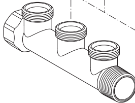
602.423.00.1, Rg, R 3/4" / Rp 3/4" 612.423.00.1, Ms, R 3/4" / Rp 3/4" 613.423.00.1, Ms, R 1" / Rp 1"
