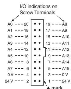
Connector Pin (male) Configuration View from engaged side
