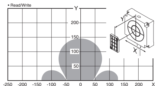
V680-H01-V2 (mounted on non-metallic material) & V680S-D8KF68 (Tag direction: Vertical)
