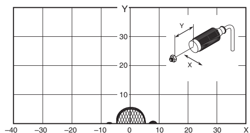
V680-D1KP52M-BT01 (mounted in metal/non-metallic material)
